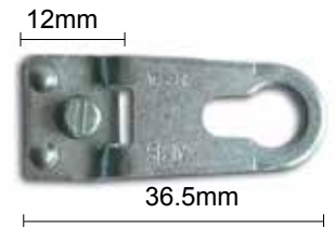
PF16 EH (PF16)
