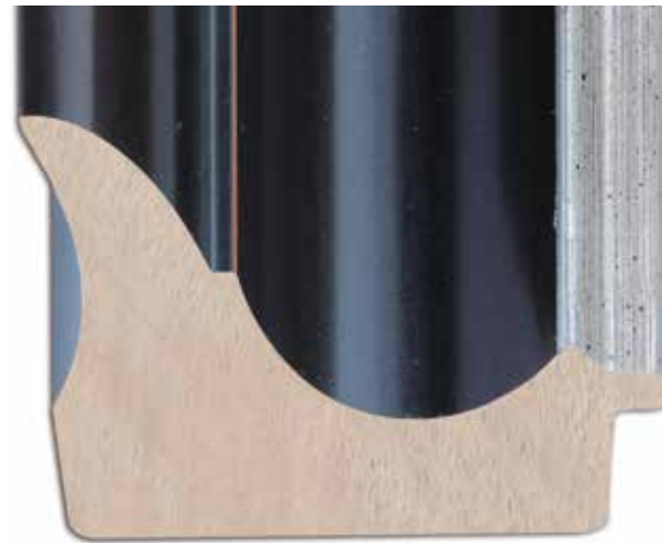
CH 9108-2 BLACK With BROWN 77W x 53H x 16RH x 7.5RW Box Quantity "20mts" PCU : 56
