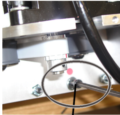
Unscrew Allen
