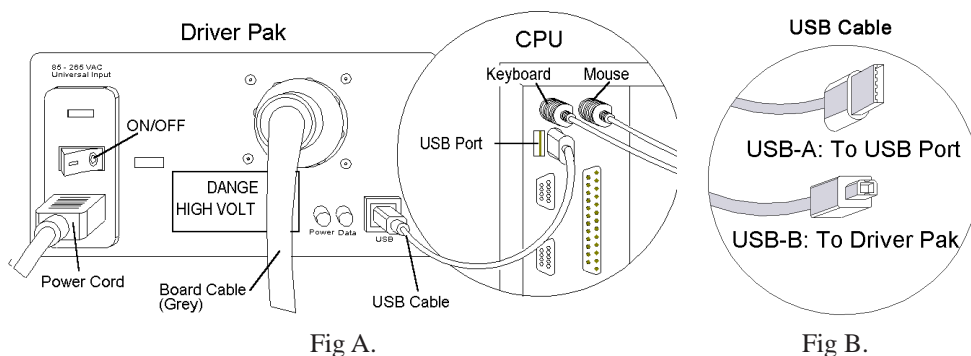
Fig A. Back of the Driver Pak and back of CPU. Fig B: Close-up of USB Cable.
