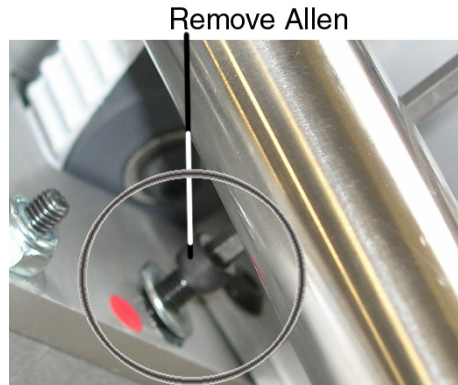
Remove Allen
